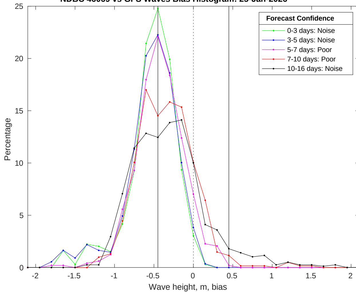
NDBC 46069 vs GFS Waves Bias Histogram: 25-Jan-2026
