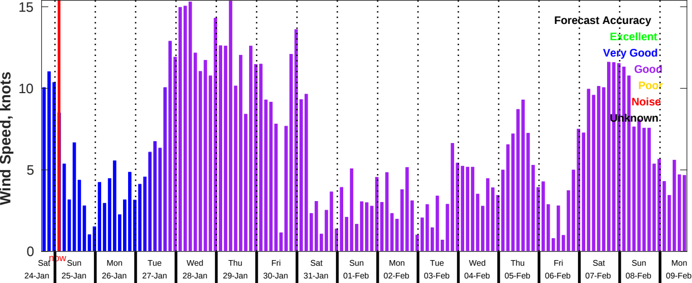
GFS Wind Speed Forecast for NDBC 46069 from 24-Jan-2026 16:00:00 to 09-Feb-2026 16:00:00
