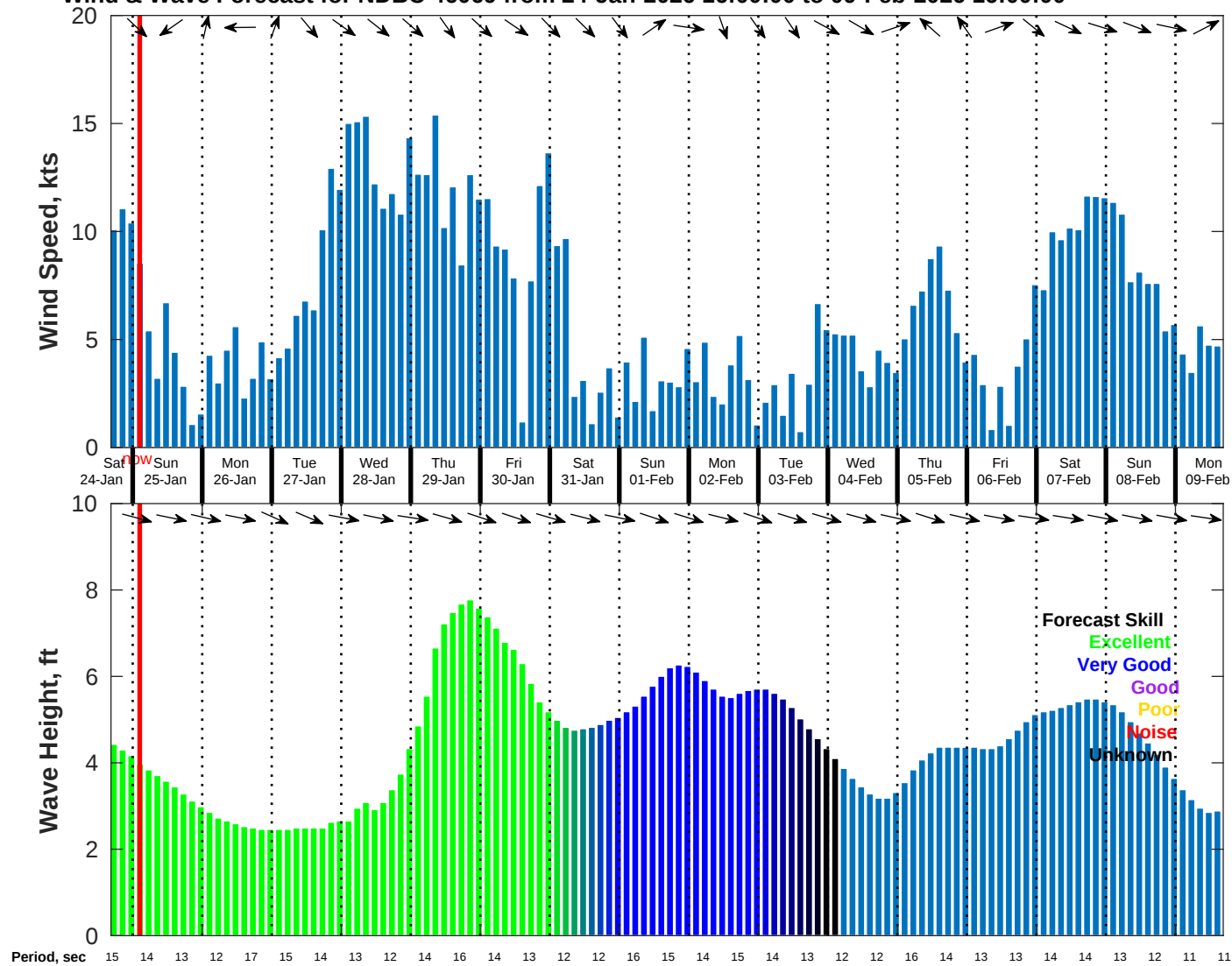
Wind & Wave Forecast for NDBC 46069 from 24-Jan-2026 16:00:00 to 09-Feb-2026 16:00:00
