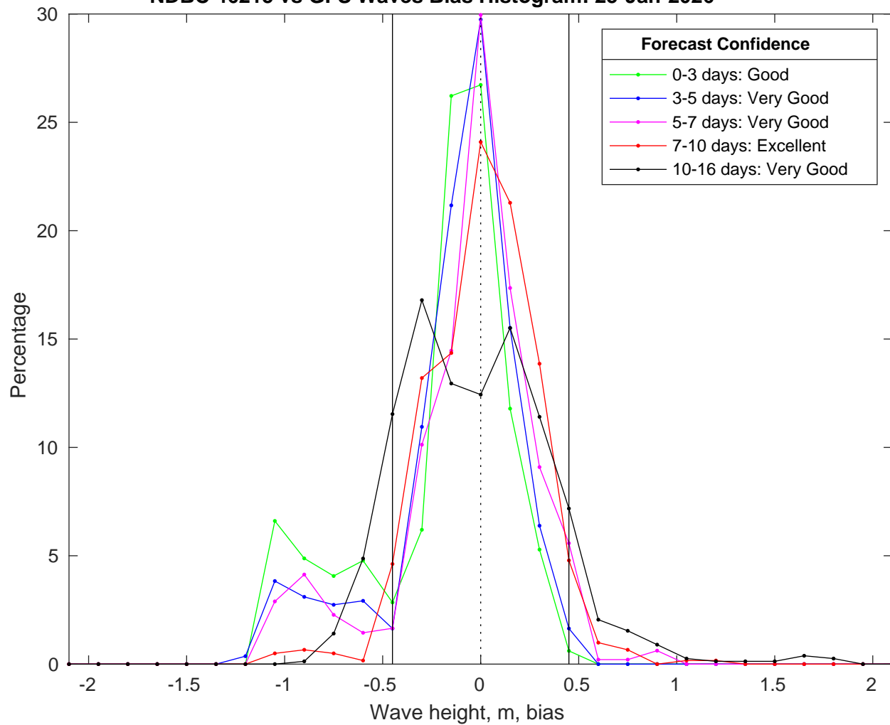
NDBC 46215 vs GFS Waves Bias Histogram: 25-Jan-2026
