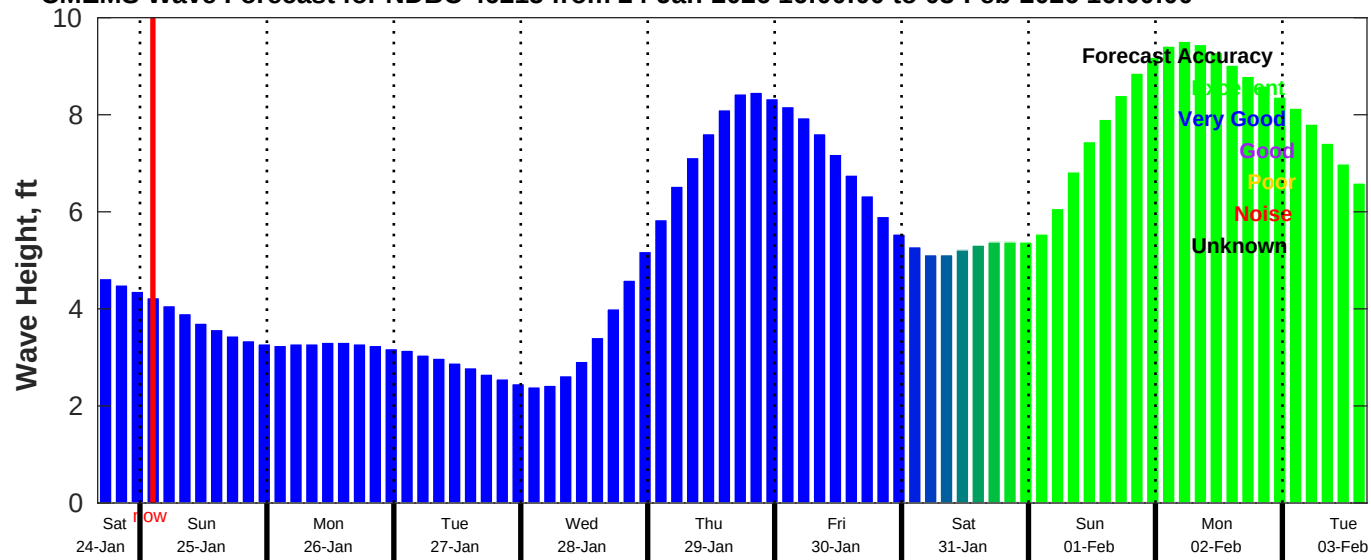
CMEMS Wave Forecast for NDBC 46215 from 24-Jan-2026 16:00:00 to 03-Feb-2026 16:00:00
