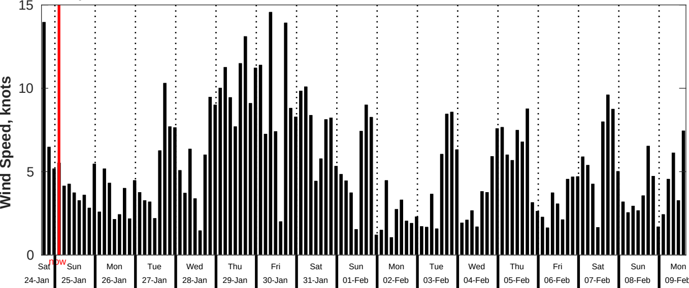
GFS Wind Speed Forecast for NDBC 46215 from 24-Jan-2026 16:00:00 to 09-Feb-2026 16:00:00
