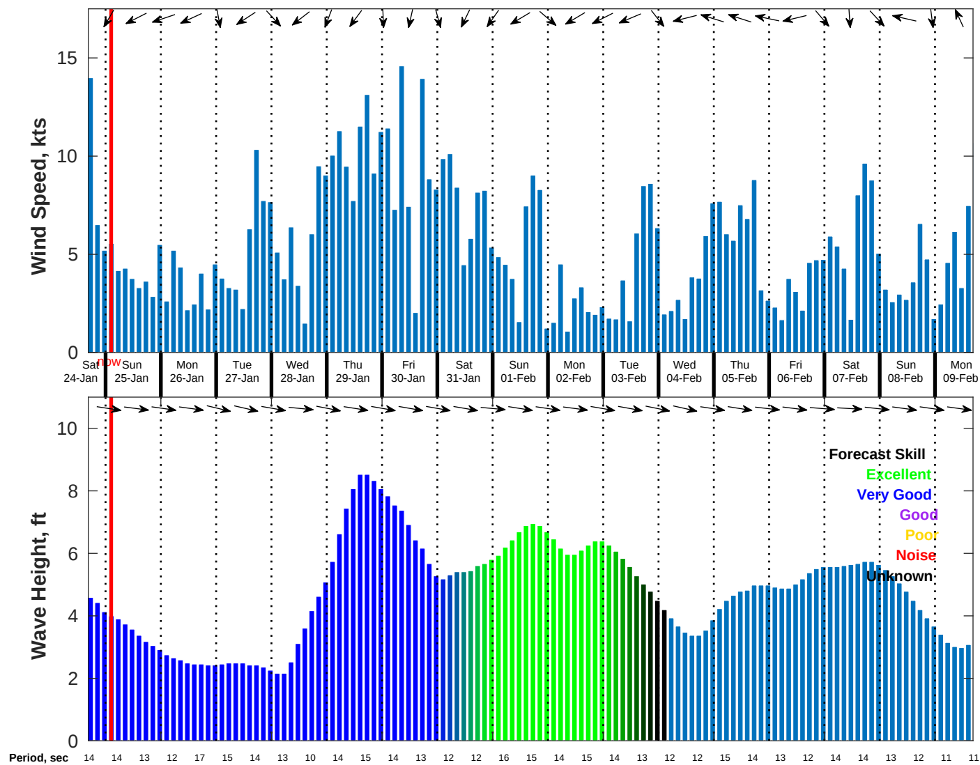
Wind & Wave Forecast for NDBC 46215 from 24-Jan-2026 16:00:00 to 09-Feb-2026 16:00:00
