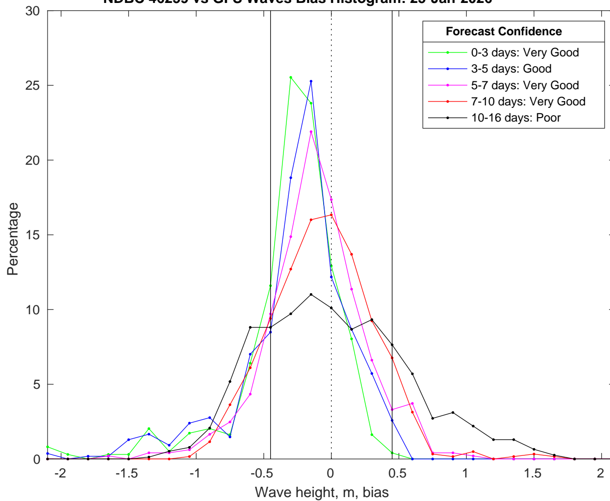
NDBC 46259 vs GFS Waves Bias Histogram: 25-Jan-2026
