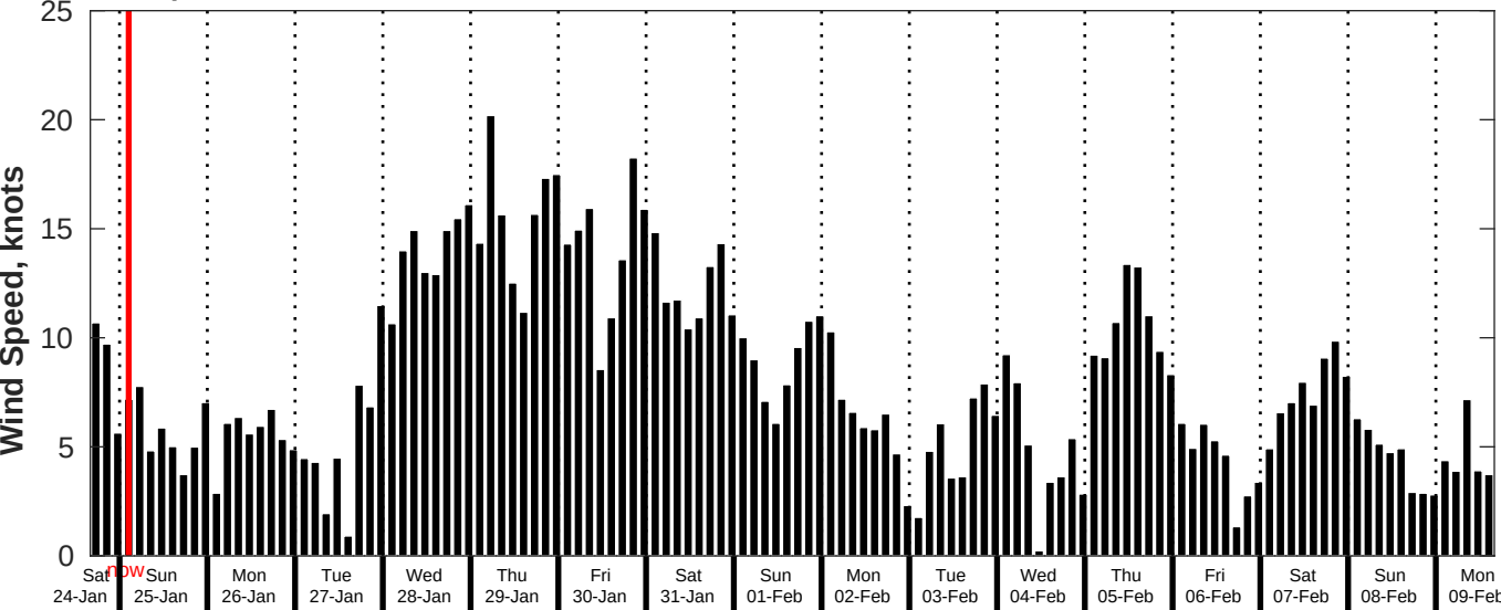
GFS Wind Speed Forecast for NDBC 46259 from 24-Jan-2026 16:00:00 to 09-Feb-2026 16:00:00
