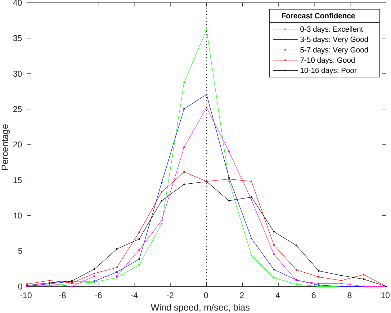
NDBC 51000 vs GFS Winds Bias Histogram: 25-Jan-2026
