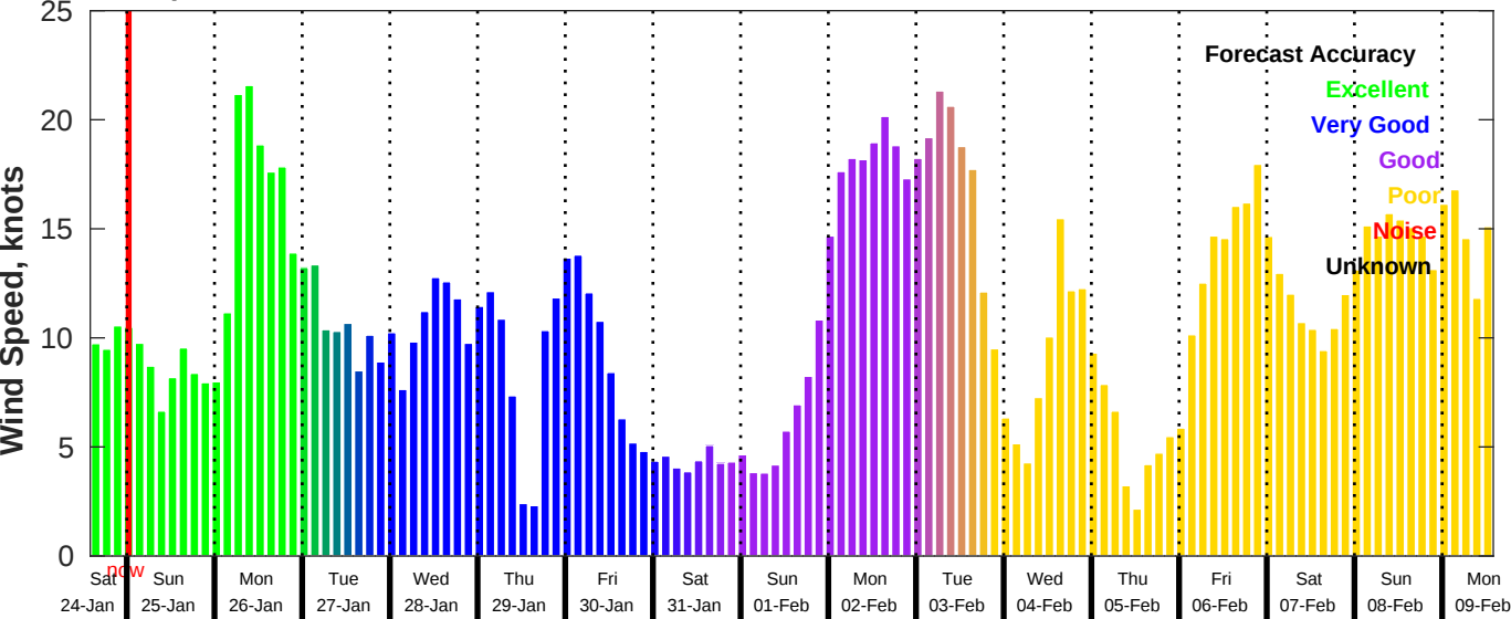
GFS Wind Speed Forecast for NDBC 51000 from 24-Jan-2026 14:00:00 to 09-Feb-2026 14:00:00
