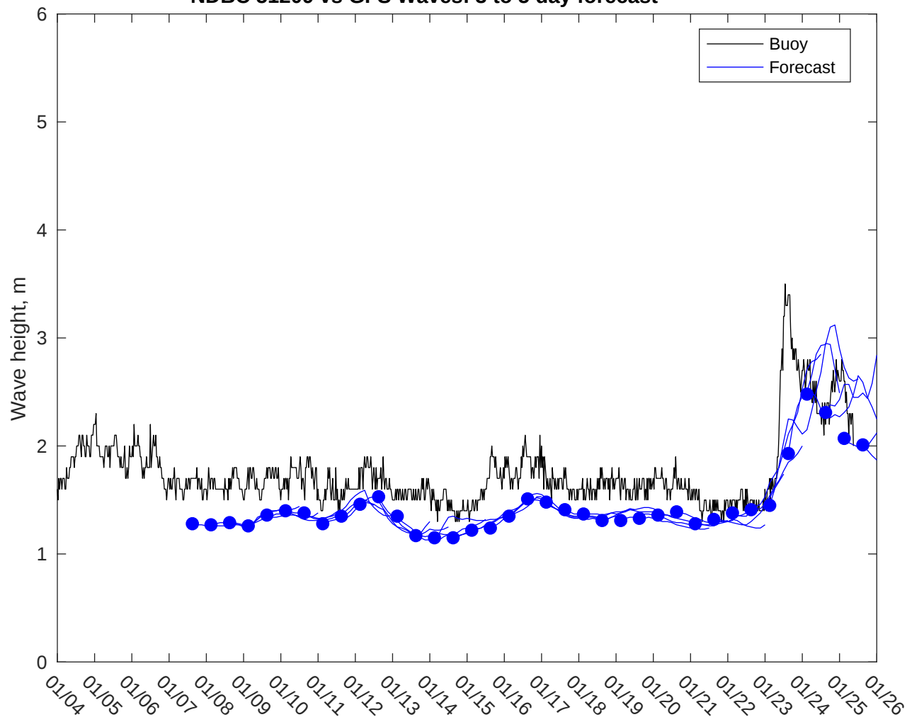
NDBC 51209 vs GFS Waves: 3 to 5 day forecast
