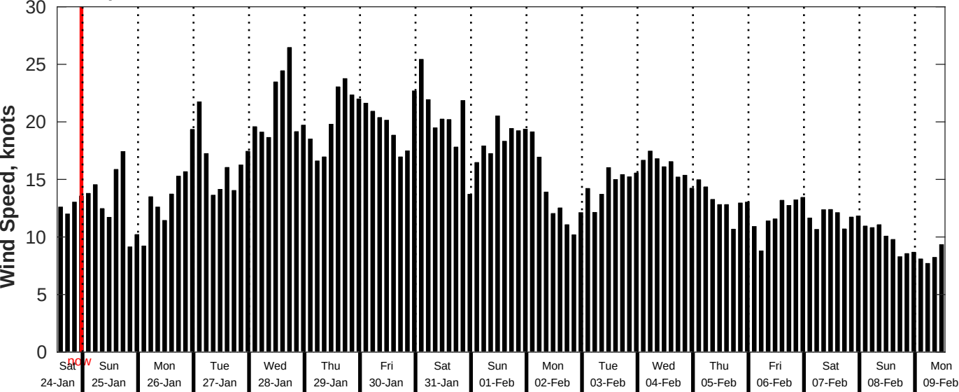
GFS Wind Speed Forecast for NDBC 51209 from 24-Jan-2026 13:00:00 to 09-Feb-2026 13:00:00
