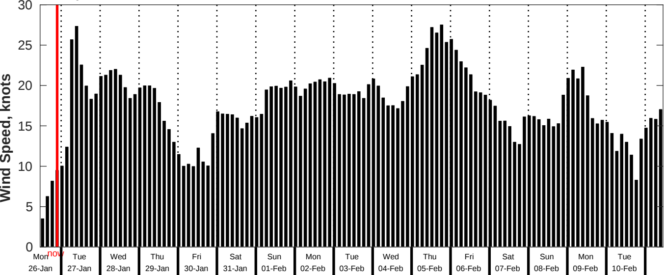
GFS Wind Speed Forecast for NDBC 52211 from 25-Jan-2026 11:00:00 to 10-Feb-2026 11:00:00
