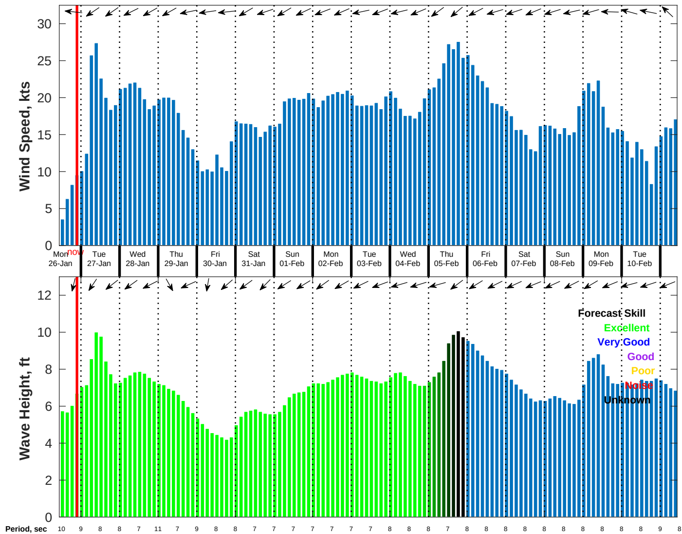
Wind & Wave Forecast for NDBC 52211 from 25-Jan-2026 11:00:00 to 10-Feb-2026 11:00:00
