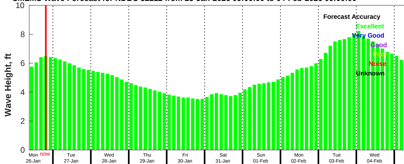
CMEMS Wave Forecast for NDBC 52212 from 25-Jan-2026 09:00:00 to 04-Feb-2026 09:00:00
