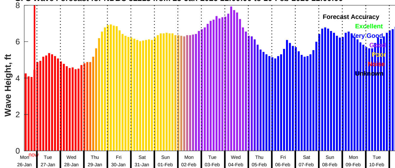
GFS Wave Forecast for NDBC 52213 from 25-Jan-2026 11:00:00 to 10-Feb-2026 11:00:00
