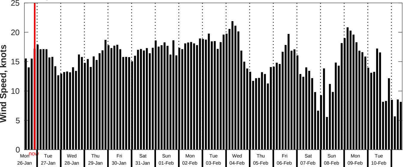
GFS Wind Speed Forecast for NDBC 52213 from 25-Jan-2026 11:00:00 to 10-Feb-2026 11:00:00
