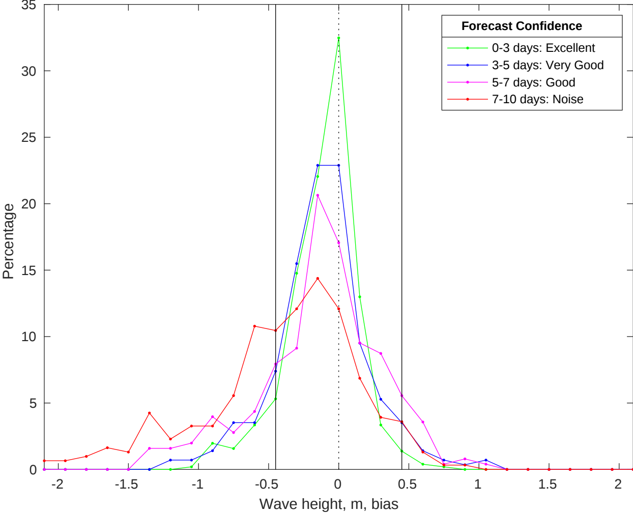
NDBC 41004 vs CMEMS Waves Bias Histogram: 26-Jan-2026
