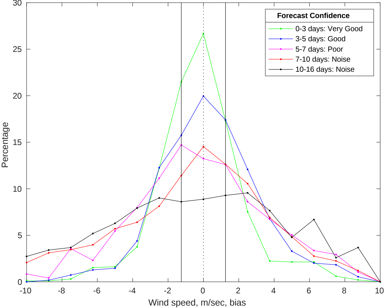
NDBC 41004 vs GFS Winds Bias Histogram: 26-Jan-2026
