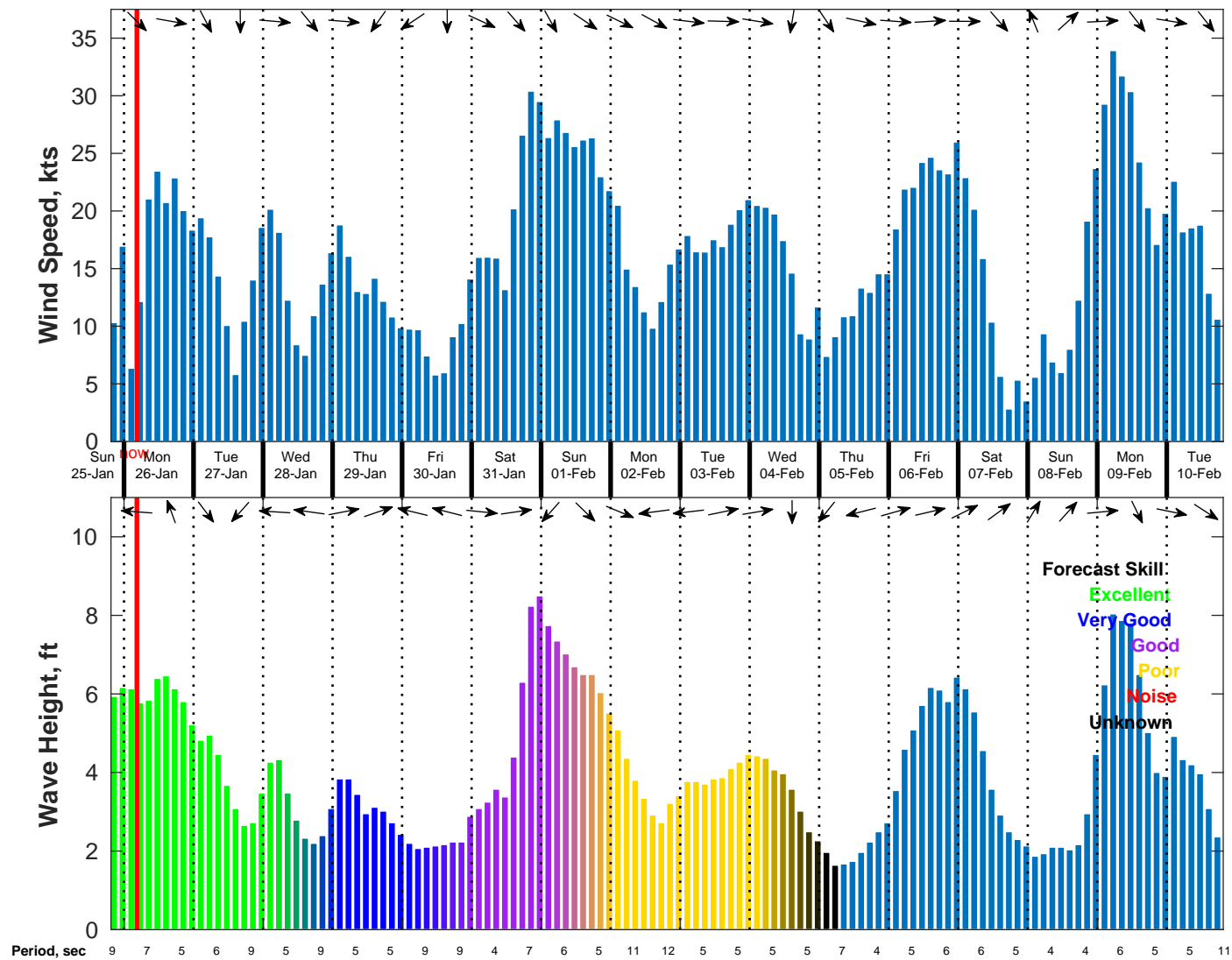
Wind & Wave Forecast for NDBC 41004 from 25-Jan-2026 19:00:00 to 10-Feb-2026 19:00:00
