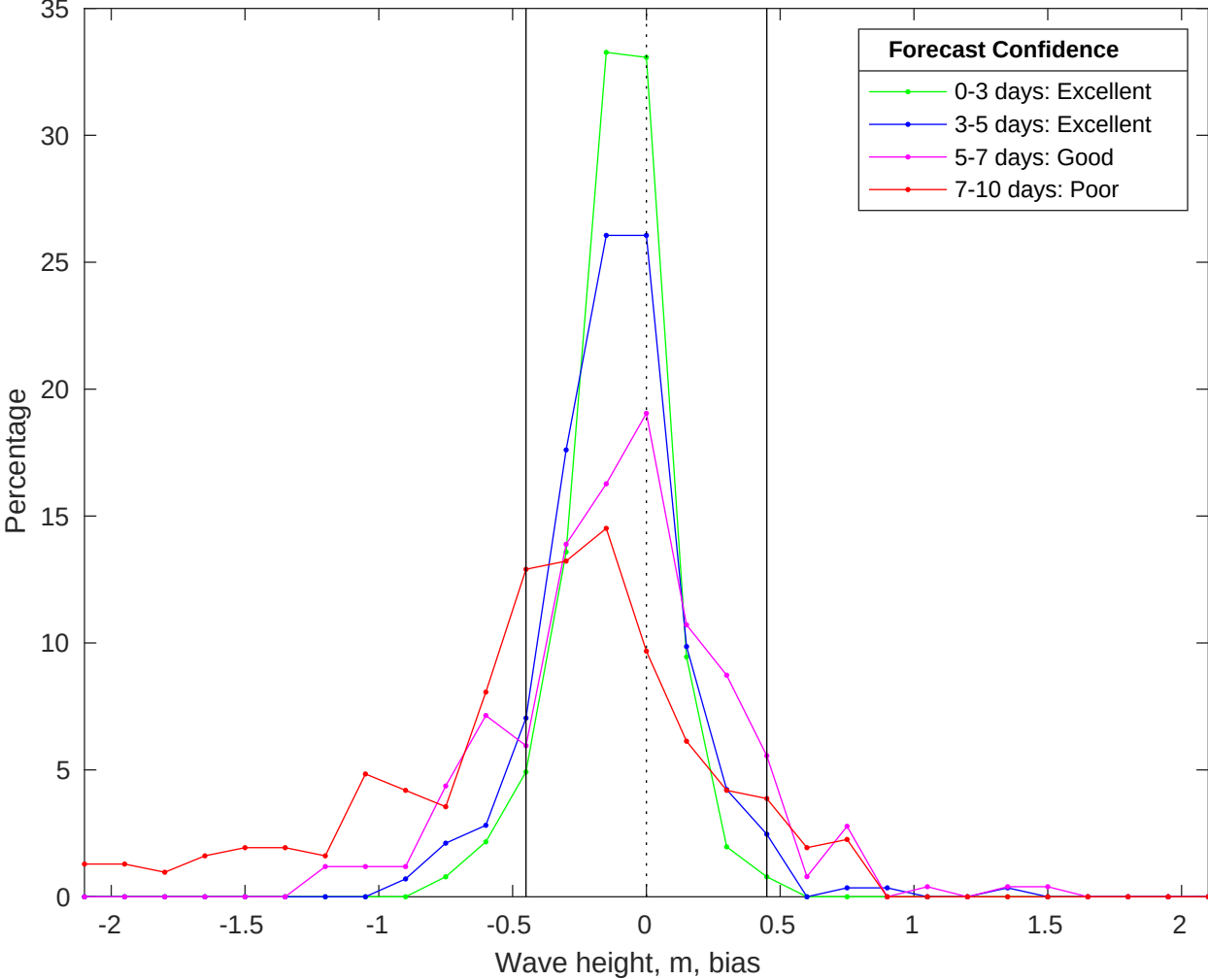
NDBC 41013 vs CMEMS Waves Bias Histogram: 26-Jan-2026
