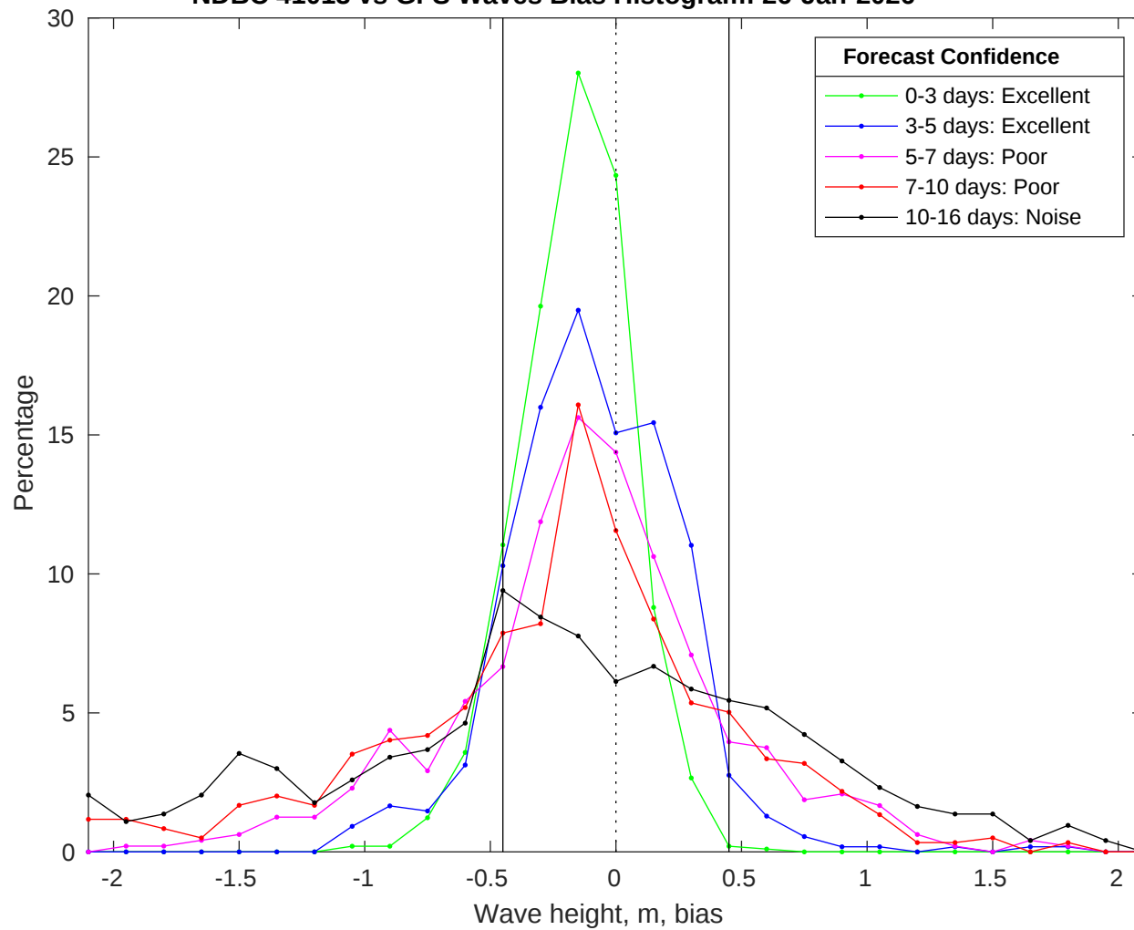
NDBC 41013 vs GFS Waves Bias Histogram: 26-Jan-2026
