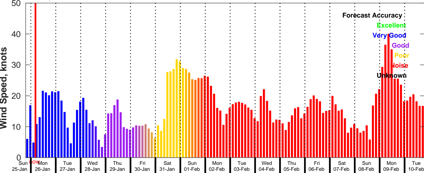
GFS Wind Speed Forecast for NDBC 41013 from 25-Jan-2026 19:00:00 to 10-Feb-2026 19:00:00
