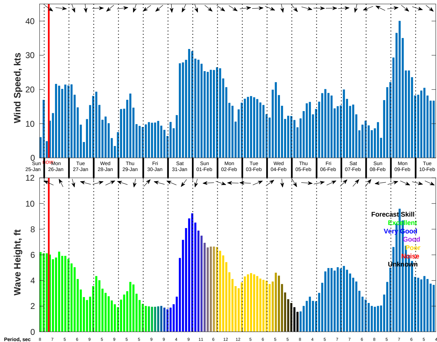
Wind & Wave Forecast for NDBC 41013 from 25-Jan-2026 19:00:00 to 10-Feb-2026 19:00:00
