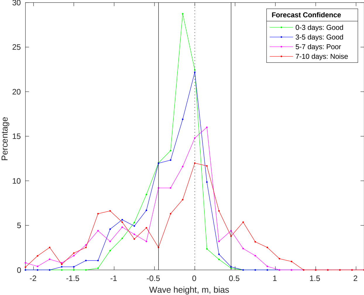
NDBC 42019 vs CMEMS Waves Bias Histogram: 26-Jan-2026
