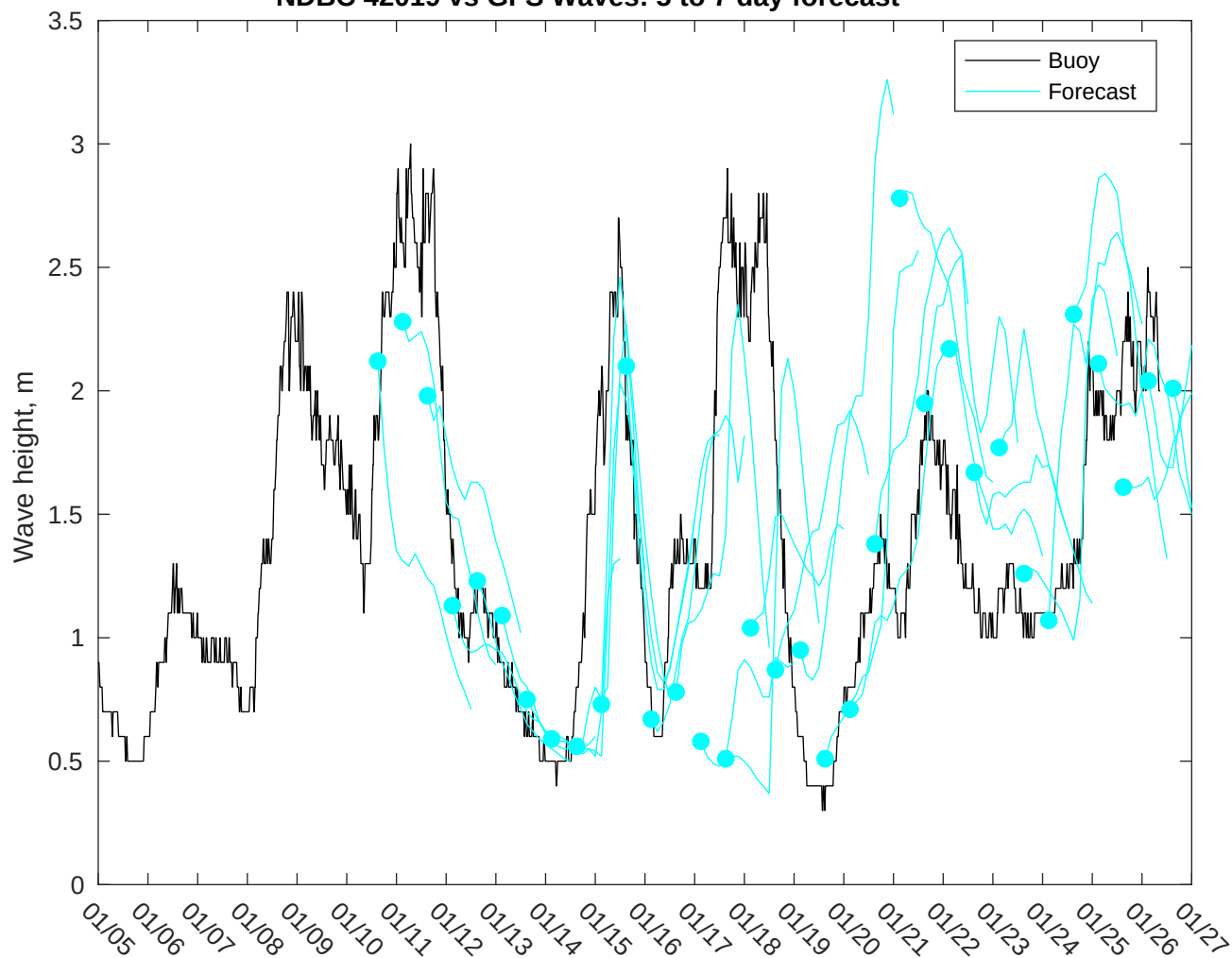
NDBC 42019 vs GFS Waves: 5 to 7 day forecast
