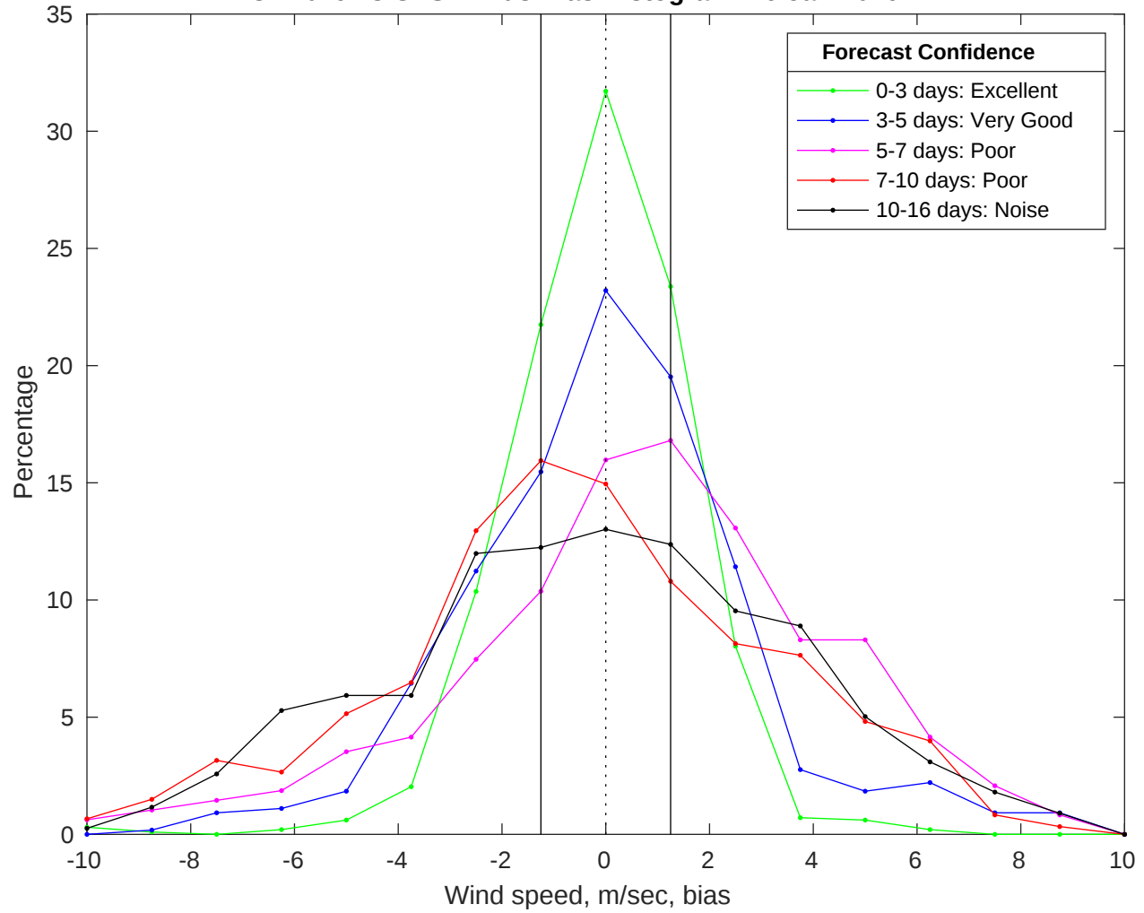
NDBC 42019 vs GFS Winds Bias Histogram: 26-Jan-2026
