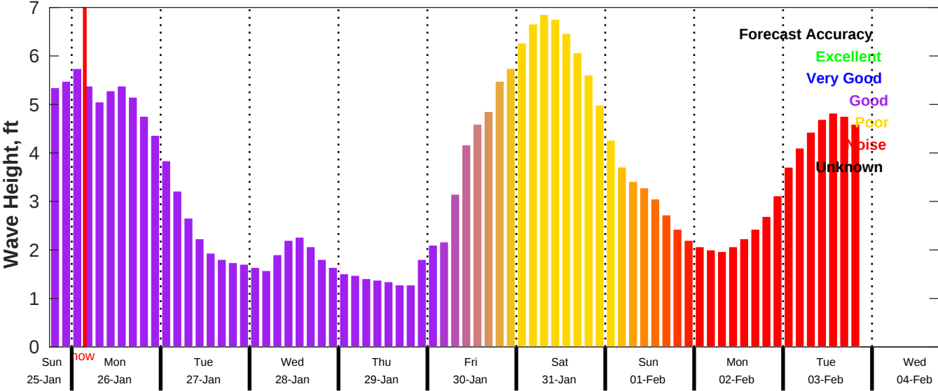
CMEMS Wave Forecast for NDBC 42019 from 25-Jan-2026 18:00:00 to 04-Feb-2026 18:00:00
