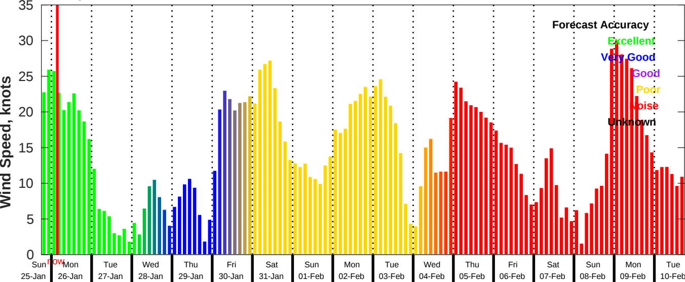
GFS Wind Speed Forecast for NDBC 42019 from 25-Jan-2026 18:00:00 to 10-Feb-2026 18:00:00
