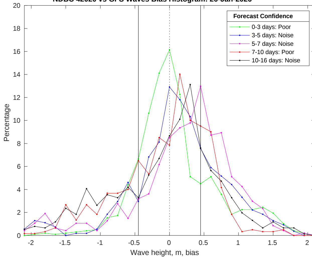
NDBC 42020 vs GFS Waves Bias Histogram: 26-Jan-2026
