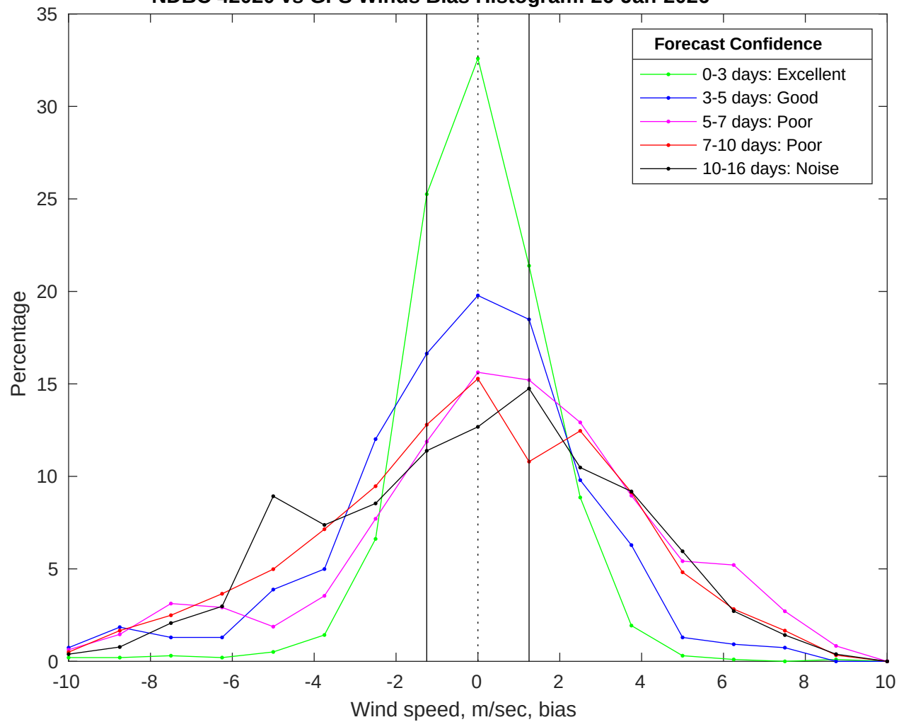
NDBC 42020 vs GFS Winds Bias Histogram: 26-Jan-2026
