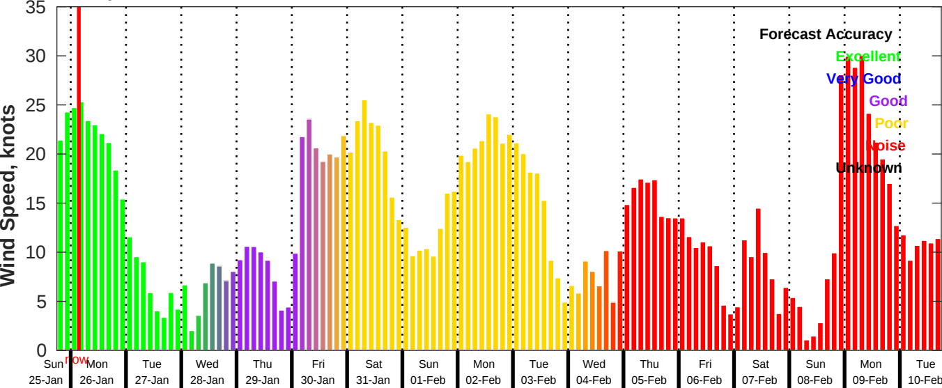
GFS Wind Speed Forecast for NDBC 42020 from 25-Jan-2026 18:00:00 to 10-Feb-2026 18:00:00
