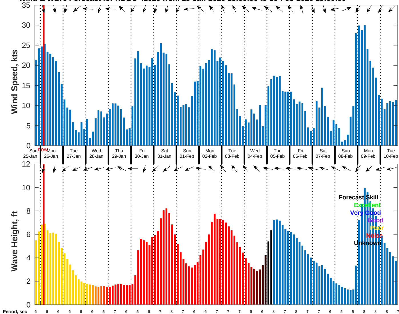
Wind & Wave Forecast for NDBC 42020 from 25-Jan-2026 18:00:00 to 10-Feb-2026 18:00:00
