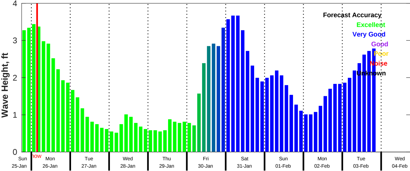
CMEMS Wave Forecast for NDBC 42035 from 25-Jan-2026 18:00:00 to 04-Feb-2026 18:00:00
