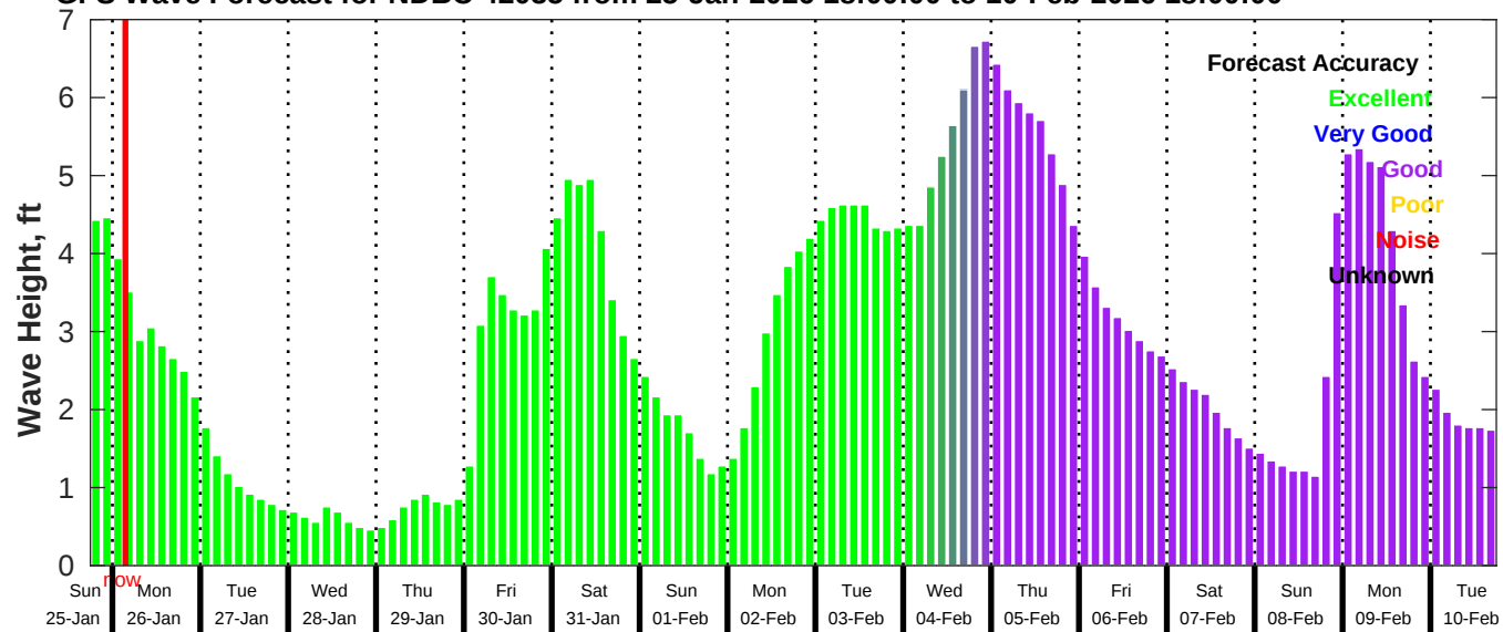
GFS Wave Forecast for NDBC 42035 from 25-Jan-2026 18:00:00 to 10-Feb-2026 18:00:00
