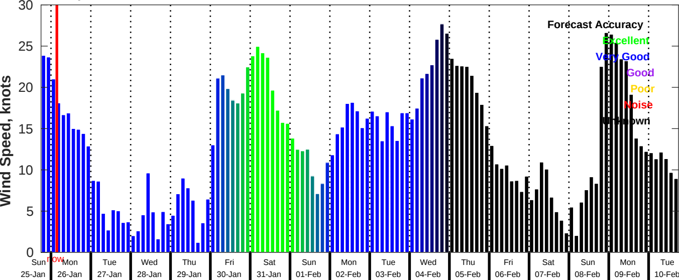
GFS Wind Speed Forecast for NDBC 42035 from 25-Jan-2026 18:00:00 to 10-Feb-2026 18:00:00
