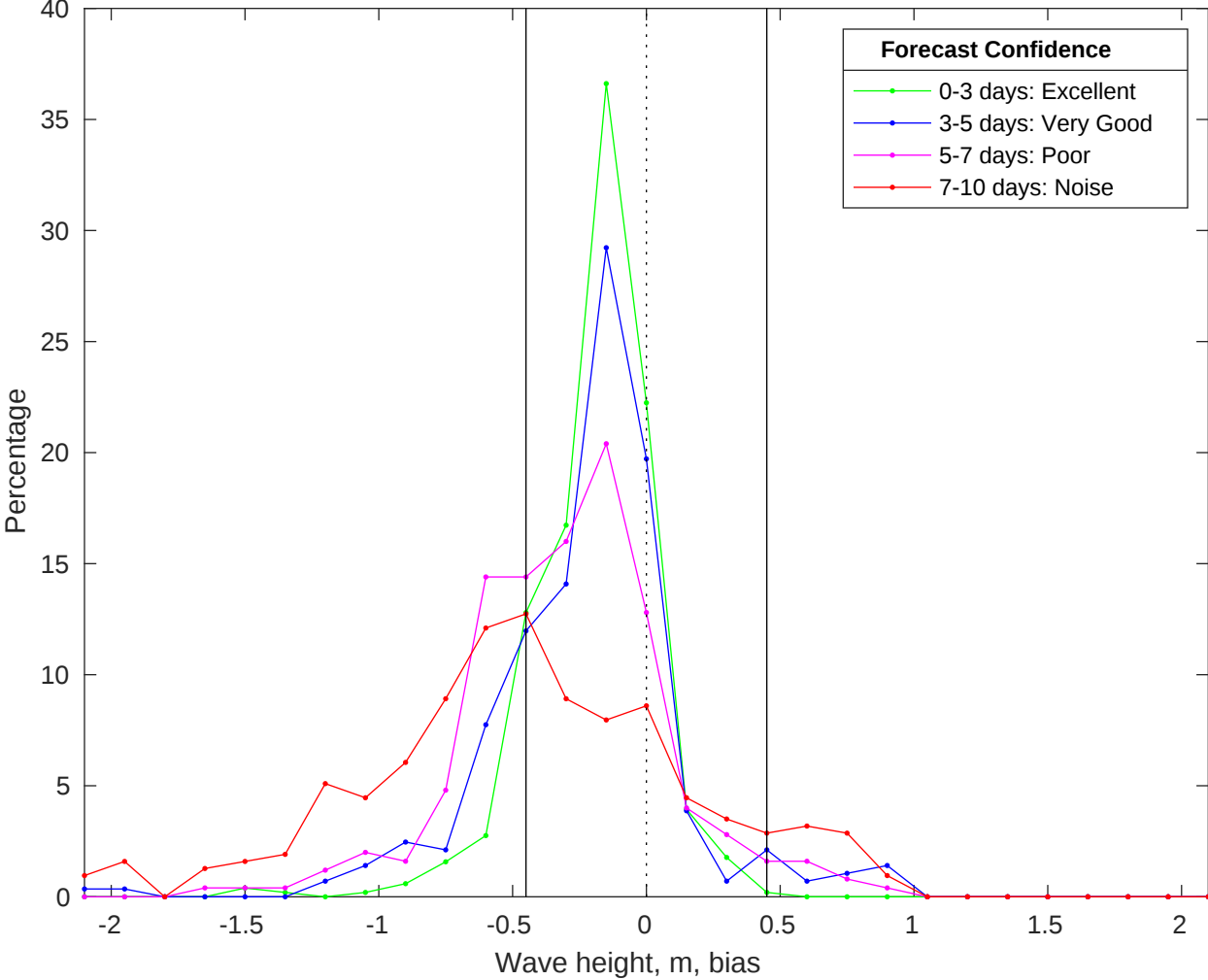
NDBC 42036 vs CMEMS Waves Bias Histogram: 26-Jan-2026
