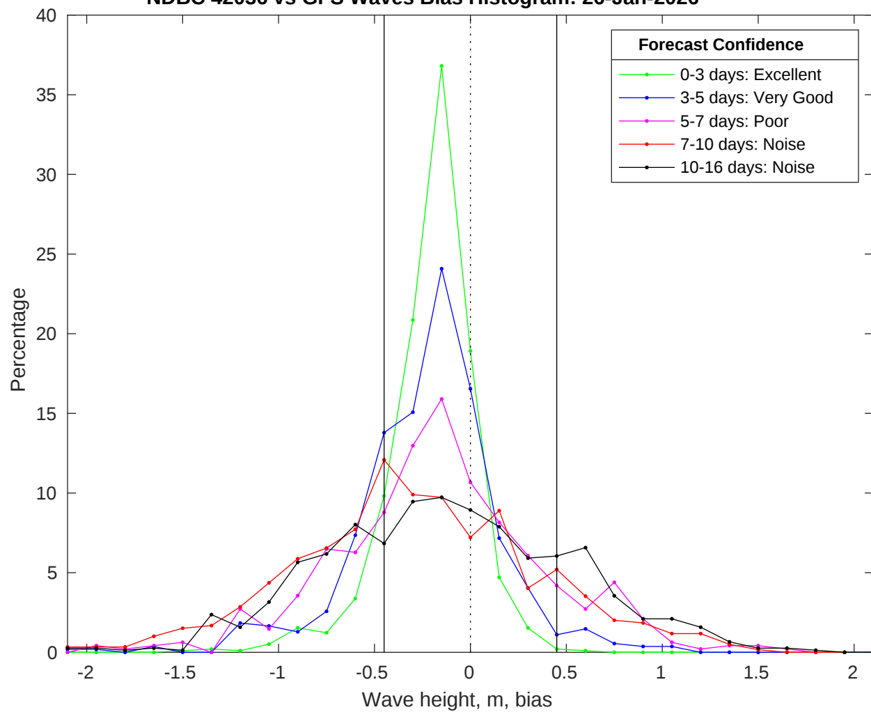
NDBC 42036 vs GFS Waves Bias Histogram: 26-Jan-2026
