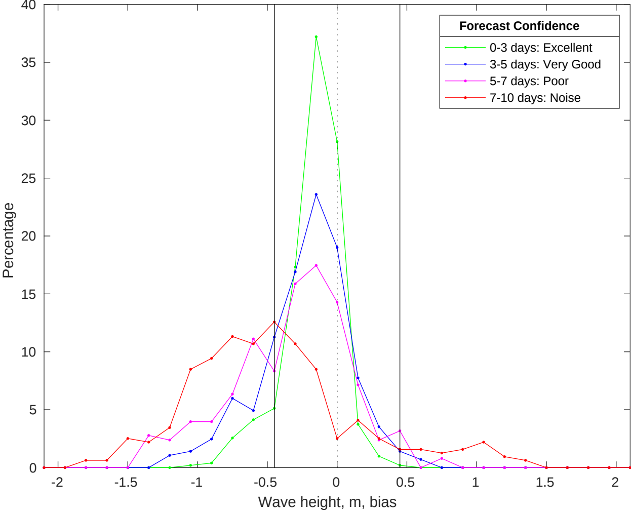
NDBC 42040 vs CMEMS Waves Bias Histogram: 26-Jan-2026
