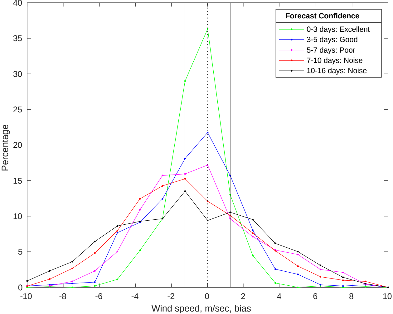
NDBC 42040 vs GFS Winds Bias Histogram: 26-Jan-2026
