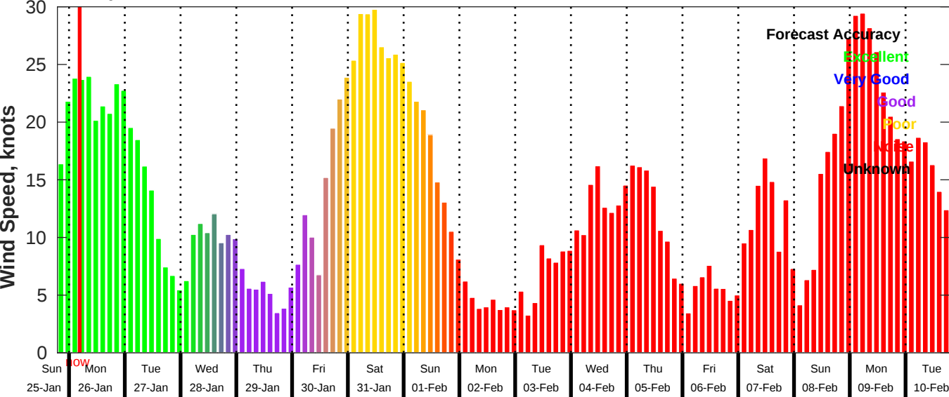
GFS Wind Speed Forecast for NDBC 42040 from 25-Jan-2026 19:00:00 to 10-Feb-2026 19:00:00
