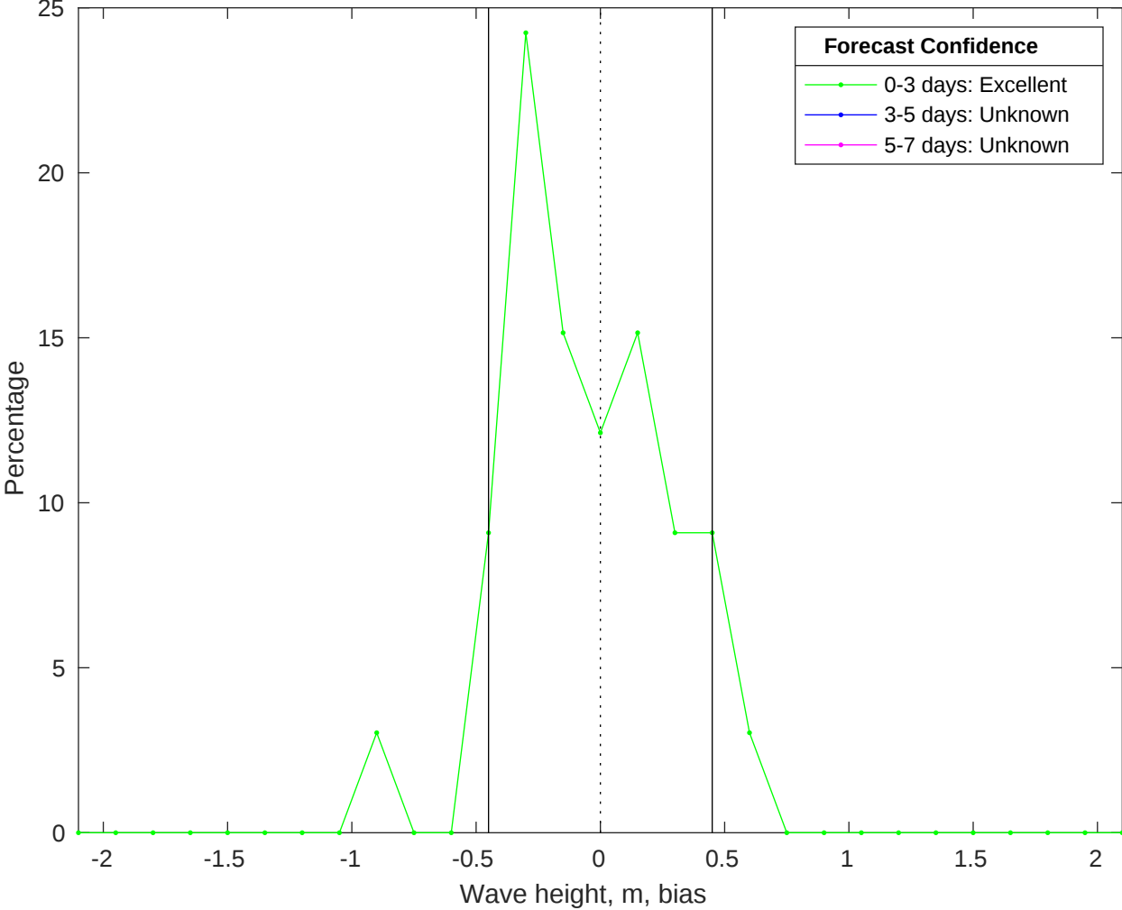
NDBC 42058 vs CMEMS Waves Bias Histogram: 26-Jan-2026
