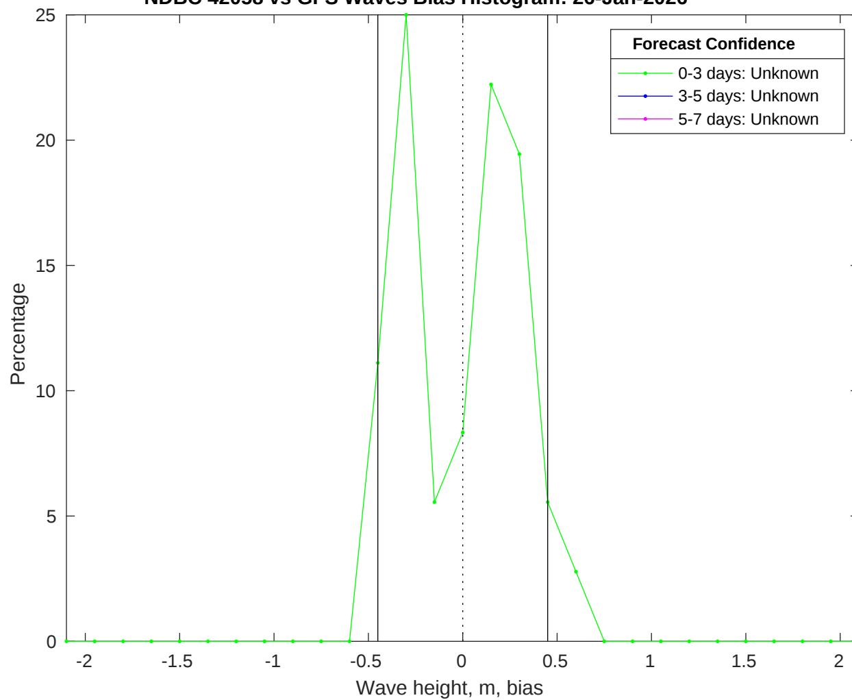
NDBC 42058 vs GFS Waves Bias Histogram: 26-Jan-2026
