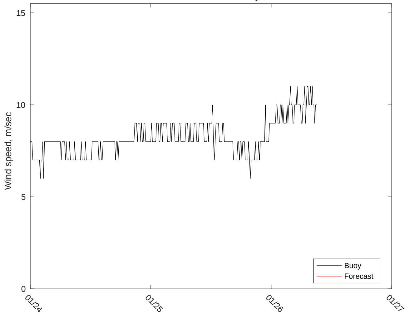
NDBC 42058 vs GFS Winds: 10 to 16 day forecast
