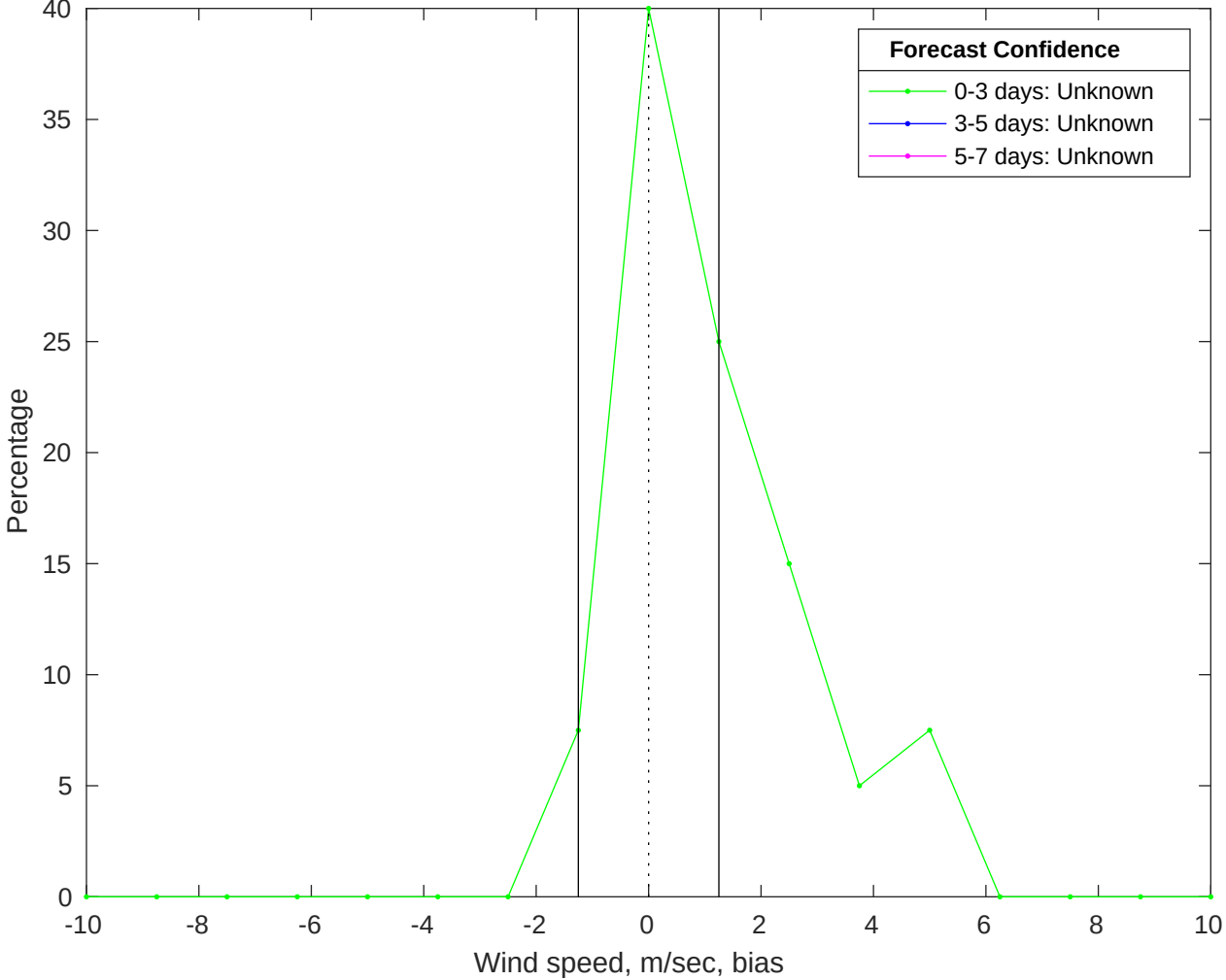
NDBC 42058 vs GFS Winds Bias Histogram: 26-Jan-2026
