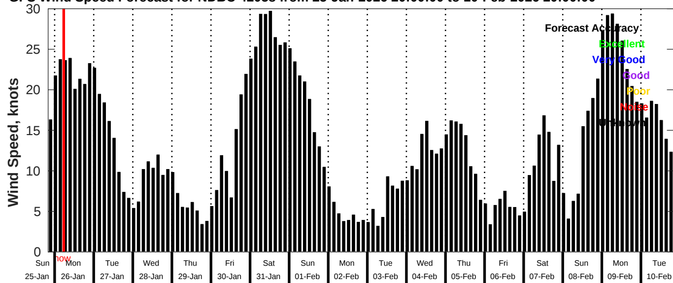
GFS Wind Speed Forecast for NDBC 42058 from 25-Jan-2026 20:00:00 to 10-Feb-2026 20:00:00
