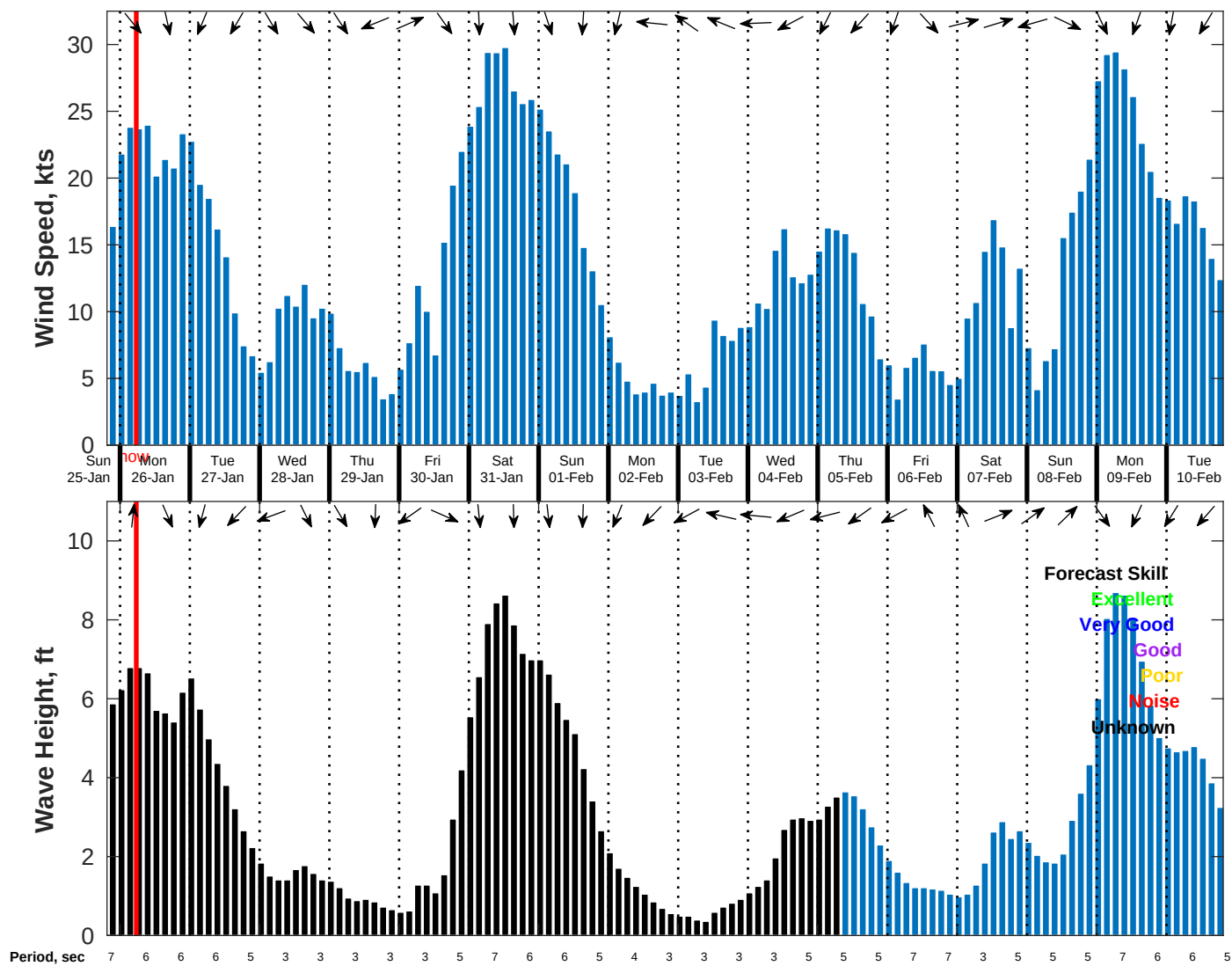
Wind & Wave Forecast for NDBC 42058 from 25-Jan-2026 20:00:00 to 10-Feb-2026 20:00:00
