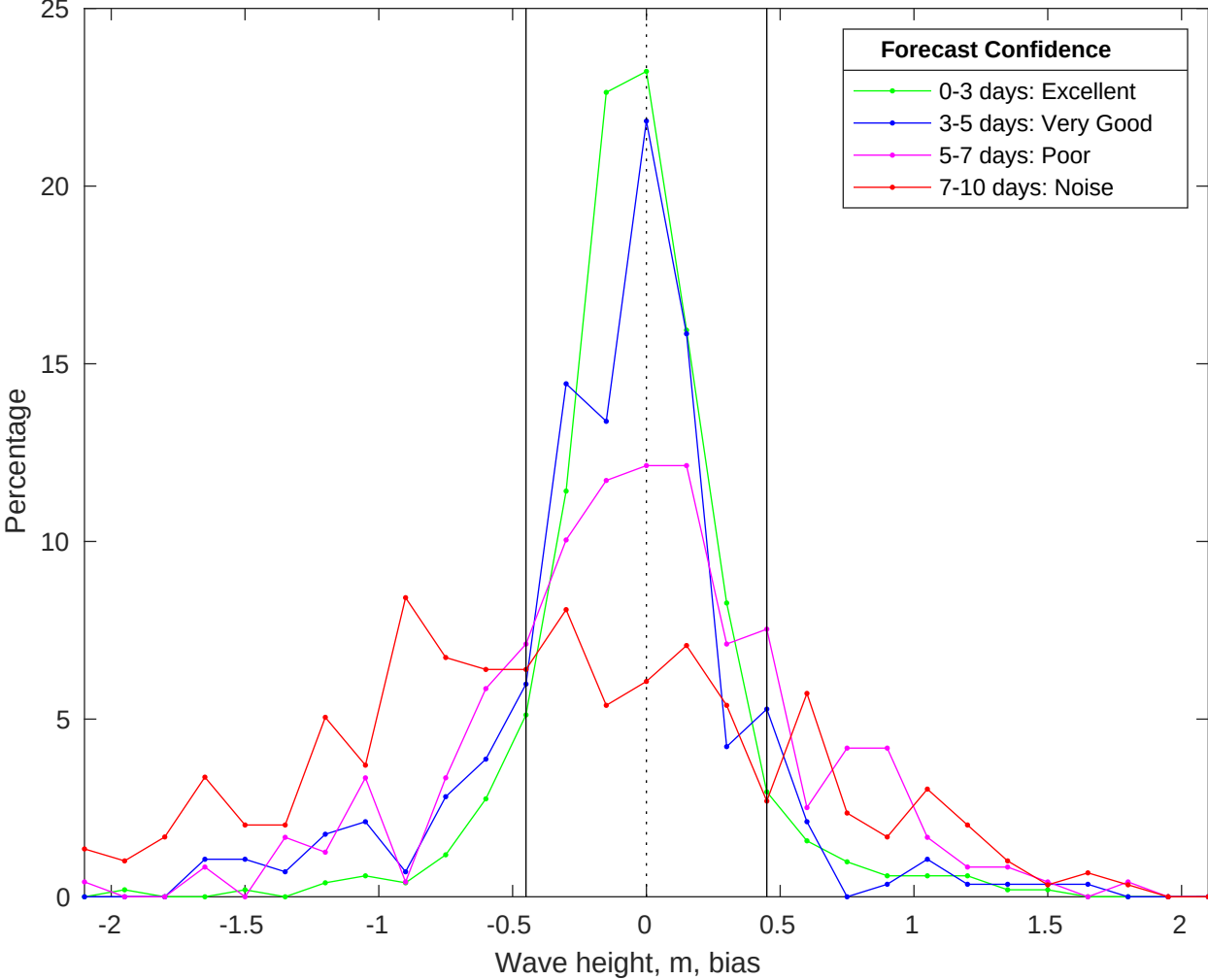
NDBC 44008 vs CMEMS Waves Bias Histogram: 26-Jan-2026
