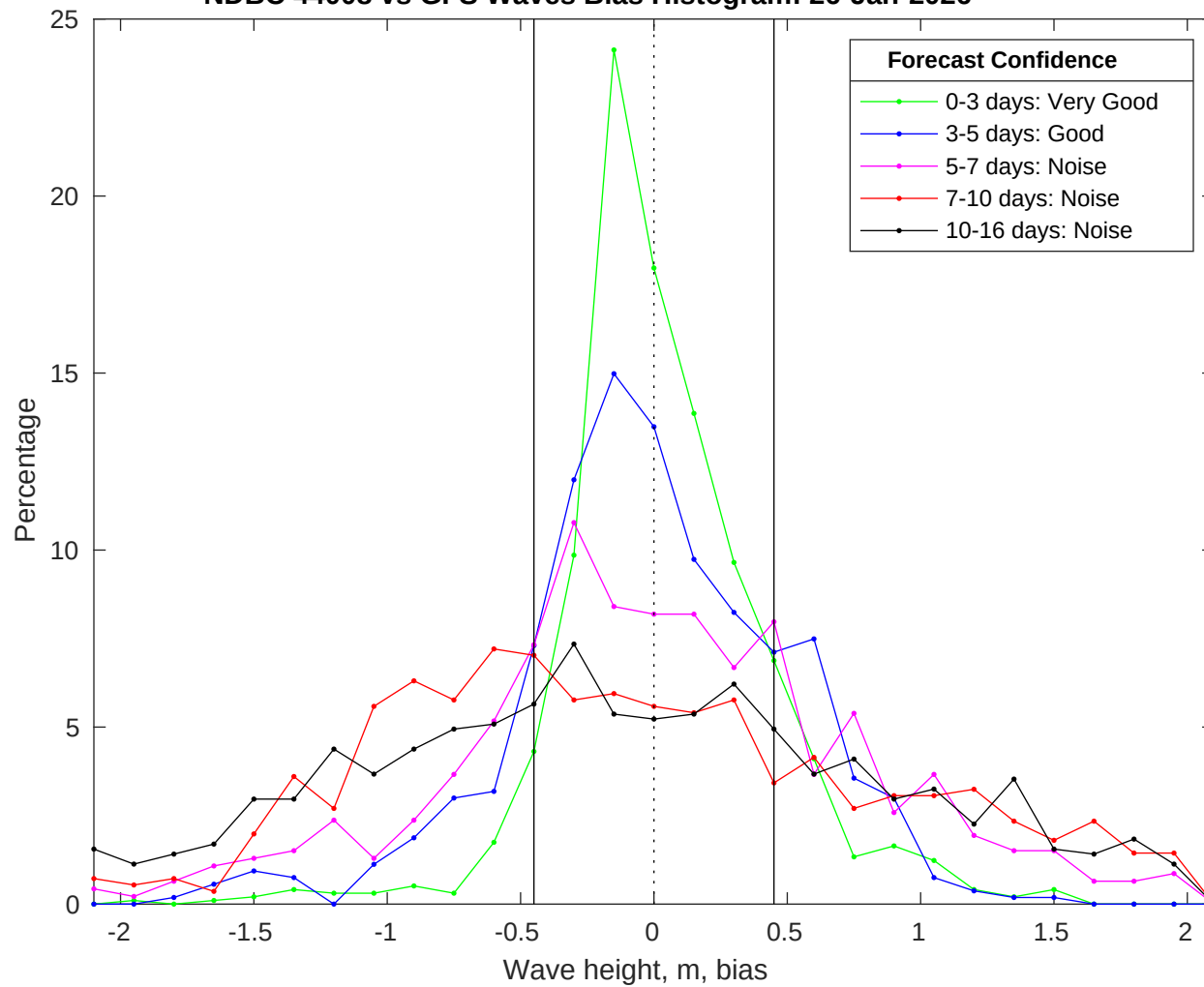
NDBC 44008 vs GFS Waves Bias Histogram: 26-Jan-2026
